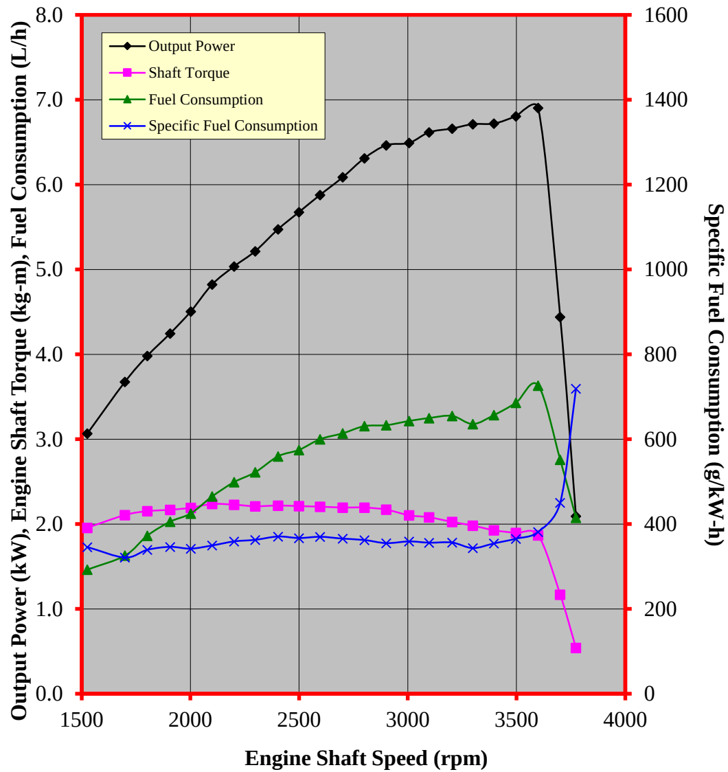
Figure 3. Performance characteristic curves of the PLATINUM KWM 399 gasoline engine
