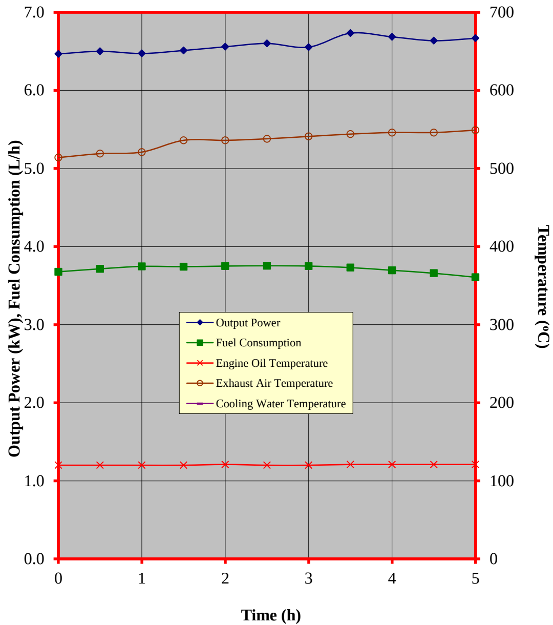
Figure 4. Performance characteristic curves during the continuous running test of the PLATINUM KWM 399 gasoline engine
